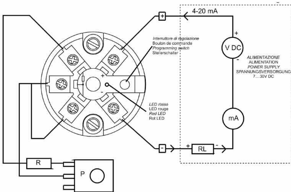
Position transmitter 4-20 mA
